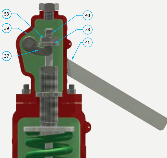
LEVER OPTION
