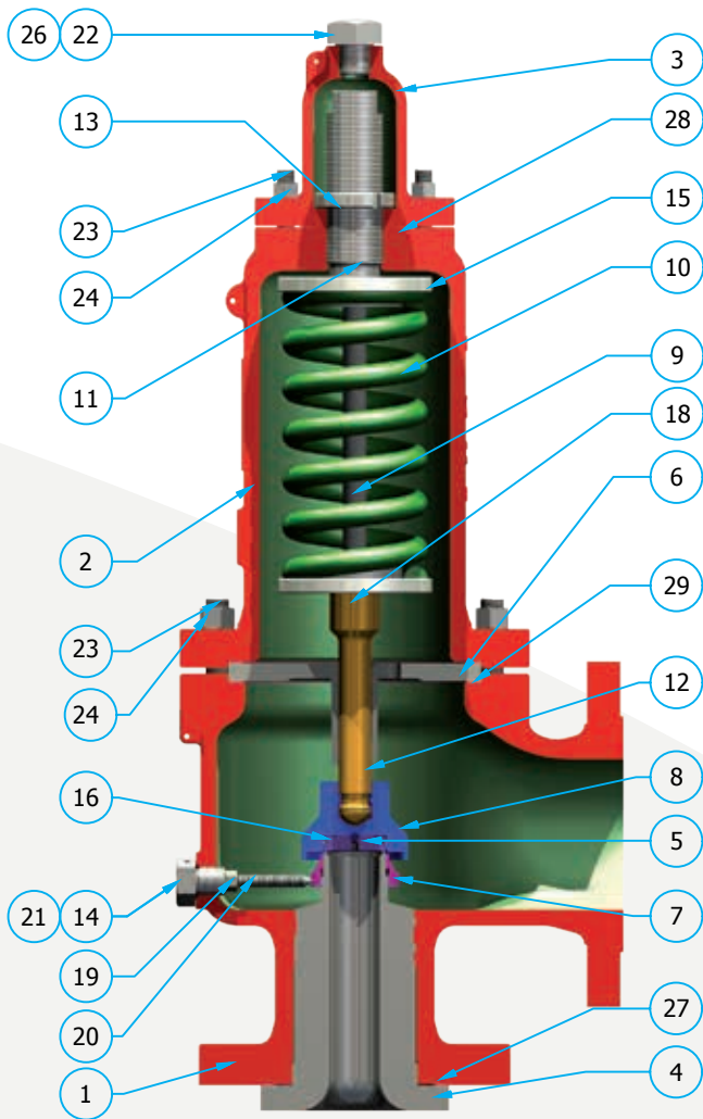
CONVENTIONALL VALVE
